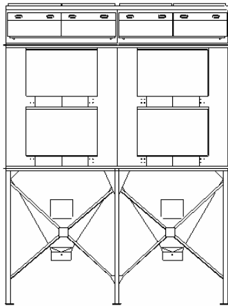
REVERSE - JET FILTERS
