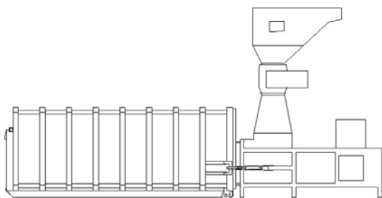
COMPACTOR & SEPARATOR ASSEMBLIES
