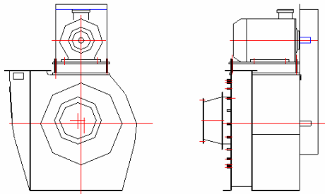
CUTTER/CONVEYOR FANS
